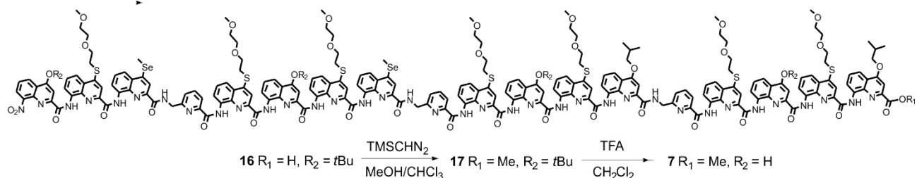
Scheme 7. Synthesis of 7 .
