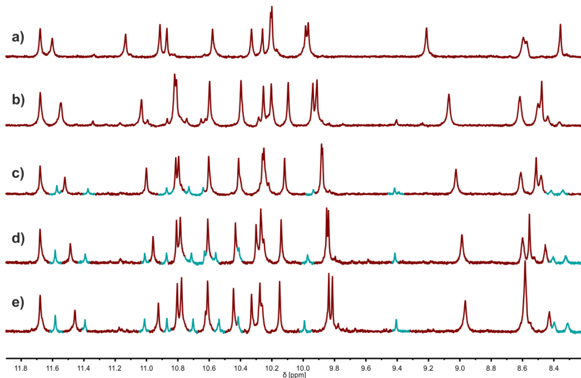
Figure S12. Interconversion of the PM and PP/MM shifted dimers of 3 upon changing \text{toluene-}d_8/\text{CD}_2\text{Cl}_2 solvent mixtures. Part of the 500 MHz ^1\text{H} NMR spectra of 3 (2.4 mM in \text{CD}_2\text{Cl}_2/\text{toluene-}d_8 mixtures) at 25 °C showing the amide and hydroxy proton resonances. The volume percentages of \text{CD}_2\text{Cl}_2 are 0 (a), 25 (b), 50 (c), 75 (d) and 100 (e). The signals of two different species are marked with different colors. The signals of two different species are marked with different colors. Signals of the species dominant in \text{CHCl}_3 ( PM shifted dimer) are marked in turquoise, those of the species dominant in \text{CH}_2\text{Cl}_2 ( PP/MM shifted dimer) are marked in brown. All spectra were measured after a 12h incubation time to reach equilibrium.
