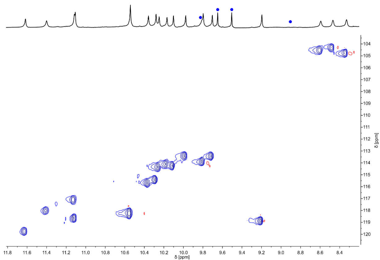
Figure S25. Identification of hydrogen bonded OH signals of 6 in \text{CD}_2\text{Cl}_2 . Part of the 500 MHz ^{15}\text{N},^1\text{H} HSQC NMR spectra (11.1 mM in \text{CD}_2\text{Cl}_2 ) at 25 °C showing the amide and hydroxy proton resonances of 6 after 2 h after pyridine-treatment. A pyridine solution of 6 was evaporated, dried and the solid was dissolved in \text{CD}_2\text{Cl}_2 and incubated for 2h prior to measuring the spectrum. Only NH resonances correlate, blue dots indicate the signals of OH protons.
