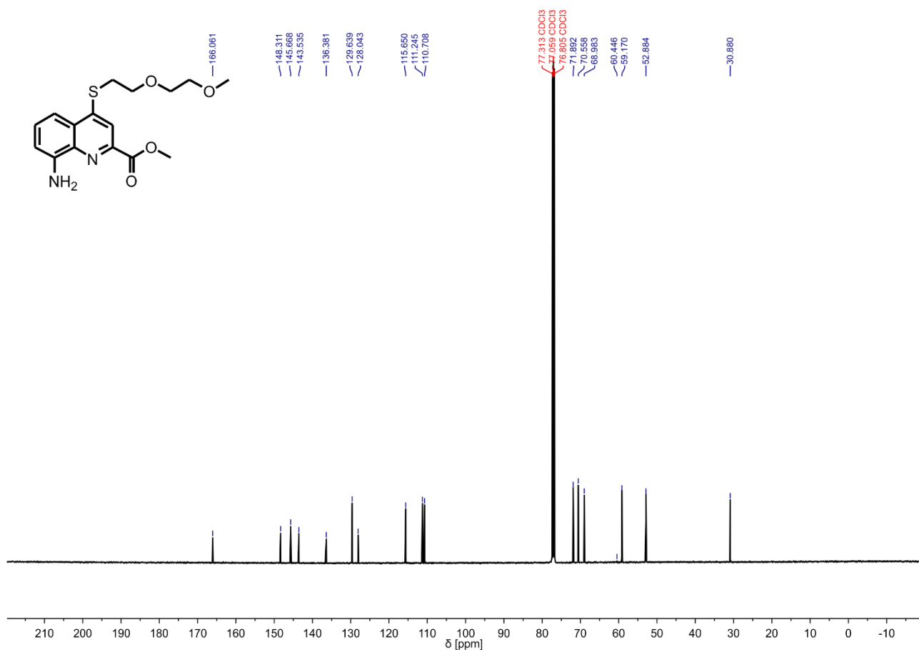
Figure S39. ^{13}\text{C} NMR spectrum (126 MHz, \text{CDCl}_3 ) of J.
