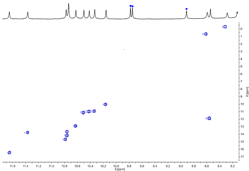
Figure S19. Identification of hydrogen bonded OH signals of 3 in (\text{CD}_2\text{Cl})_2 . Part of the 500 MHz ^{15}\text{N}, ^1\text{H} HSQC NMR spectrum of 3 (4.4 mM in (\text{CD}_2\text{Cl})_2 ) at 25 °C showing the amide and hydroxy proton resonances. Only NH resonances correlate, blue dots indicate the signals of OH protons. The spectrum was measured after a two-hour incubation time to reach equilibrium.
