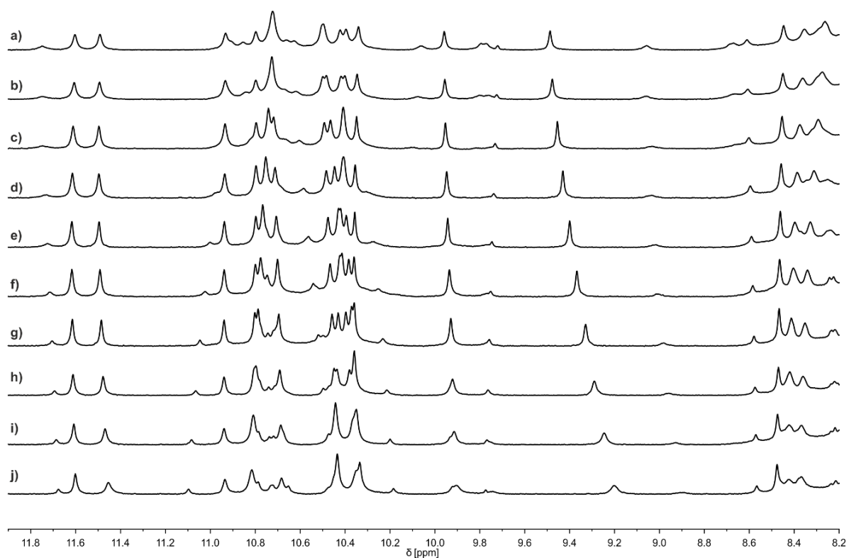
Figure S17. The proportions of the PM and PP/MM shifted dimers of 3 do not depend on temperature. Part of the 400 MHz ^1\text{H} NMR spectra of 3 (2.5 mM in (\text{CDCl}_2)_2 ) showing the amide and hydroxy proton resonances at 25 °C (a), 30 °C (b), 40 °C (c), 50 °C (d), 60 °C (e), 70 °C (f), 80 °C (g), 90 °C (h), 100 °C (i), and 110 °C (j). The initial spectrum was measured after a two-week incubation time to reach equilibrium. Between each other measurement the sample was equilibrated for 15 min.
