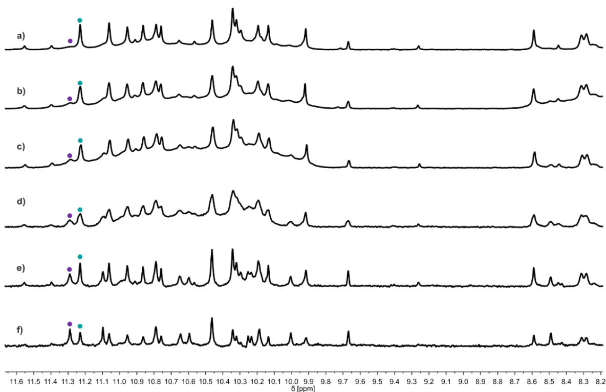
Figure S7. Solution NMR estimation of the dissociation constant of 3_2 . Part of the 500 MHz ^1\text{H} NMR spectra of 3 (in 10:90 \text{DMSO-}d_6/\text{CDCl}_3 ) at 25 °C showing the amide and hydroxy proton resonances. The total concentration of the sample was 2.44 mM (a), 1.22 mM (b), 0.61 mM (c), 0.30 mM (d), 0.15 mM (e), and 0.076 mM (f). The signals whose integration was used for the determination of the dissociation constant are marked in turquoise and violet. The ratio of monomer to dimer is 10:100 (a), 22:100 (b), 42:100 (c), 92:100 (d), 140:100 (e), 260:100 (f). Thus, the concentration of monomer in solution is 0.12 mM (a), 0.12 mM (b), 0.11 mM (c), 0.095 mM (d), 0.062 mM (e) and 0.043 mM (f). The concentration of dimer in solution is 1.16 mM (a), 0.55 mM (b), 0.25 mM (c), 0.103 mM (d), 0.044 mM (e), 0.017 mM (f). The dissociation constant was calculated using the following equation: K = \frac{[\text{Monomer}]^2}{[\text{Dimer}]} . The value of the dissociation constant equals 1.24 \times 10^{-5} (a), 2.62 \times 10^{-5} (b), 4.84 \times 10^{-5} (c), 8.76 \times 10^{-5} (d), 8.73 \times 10^{-5} (e) and 1.09 \times 10^{-4} M (f) leading to an average dissociation constant K_d of 62 \mu\text{M} . All spectra were measured after a two-week incubation time to reach equilibrium.
