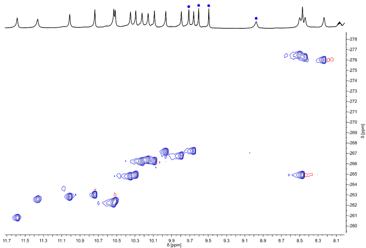
Figure S20. Identification of hydrogen bonded OH signals of 4 in \text{CD}_2\text{Cl}_2 . Part of the 500 MHz ^{15}\text{N}, ^1\text{H} HSQC NMR spectrum of 4 (7.02 mM in \text{CD}_2\text{Cl}_2 ) 25 °C showing the amide and hydroxy proton resonances. Only NH resonances correlate, blue dots indicate the signals of OH protons. A pyridine solution of 4 was evaporated, dried and the solid was dissolved in \text{CD}_2\text{Cl}_2 and incubated for four weeks prior to measuring the spectrum.
