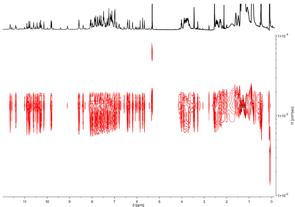
Figure S18. The PM and PPIMM shifted dimers of 3 have the same hydrodynamic radius. 500 MHz ^1\text{H} DOSY spectrum of 3 (5 mM in \text{CD}_2\text{Cl}_2 ) at 25 °C. The spectrum was measured after a two-hour incubation time to reach equilibrium.
