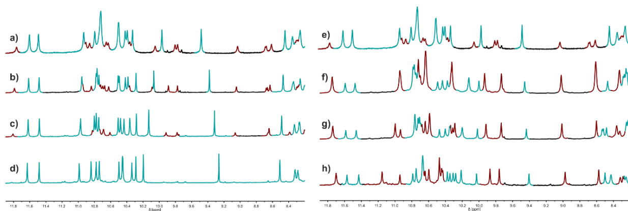
Figure S13. Interconversion of the PM and PP/MM shifted dimers of 4 upon changing \text{CDCl}_3/(\text{CDCl}_2)_2/\text{CD}_2\text{Cl}_2 solvent mixtures. a)-d) Part of the 500 MHz ^1\text{H} NMR spectra of 3 (2.4 mM in \text{CDCl}_3/(\text{CDCl}_2)_2 mixtures) at 25 °C showing the amide and hydroxy proton resonances. The volume percentages of (\text{CDCl}_2)_2 are 100 (a), 75 (b), 50 (c), and 25 (d). e)-f) Part of the ^1\text{H} NMR spectra (500 MHz, 25 °C) showing the amide and hydroxy proton resonances of 3 at 2.4 mM in \text{CD}_2\text{Cl}_2/(\text{CDCl}_2)_2 mixtures. The volume percentages of (\text{CDCl}_2)_2 are 100 (e), 75 (f), 50 (g), and 25 (h). The signals of two different species are marked with different colors. Signals of the species dominant in \text{CHCl}_3 ( PM shifted dimer) are marked in turquoise, those of the species dominant in \text{CH}_2\text{Cl}_2 ( PP/MM shifted dimer) are marked in brown. All spectra were measured after a 2h incubation time to reach equilibrium.
