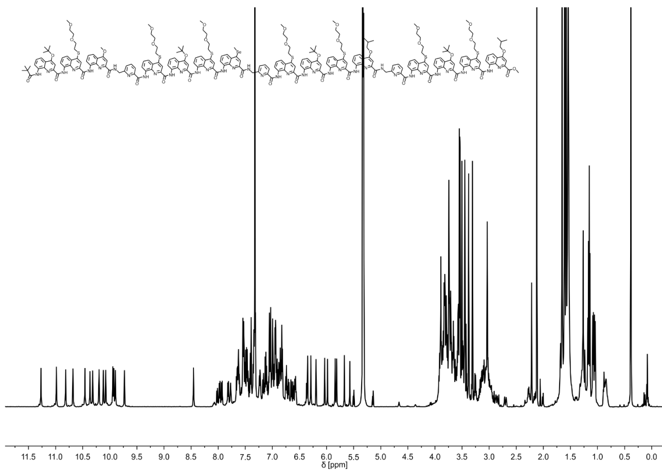
Figure S46. 1 H NMR spectrum (500 MHz, CD 2 Cl 2 ) of 11 .
