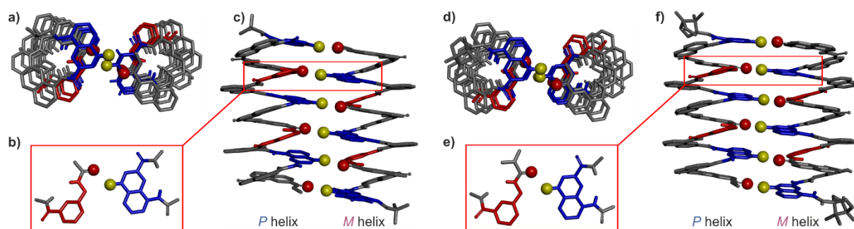
Figure S4. Crystal structures of 3 and 5 from chloroform. Top view (a) and side view (c) of the solid state structure of 3 obtained from crystals grown from \text{CHCl}_3 . The prevalent hydrogen-bonding pattern is shown in (b). Top view (d) and side view (f) of the pseudo-racemic solid state structure of 5 obtained from crystals grown from \text{CHCl}_3 (a pseudo center of inversion applies to the helices but not to the camphanyl groups). The prevalent hydrogen-bonding pattern is shown in (e). Both structures show a PM shifted dimer. The hydrogen-bonding donor and acceptors are shown as yellow and red balls, respectively. The X units are shown in blue and the P Units in red tubes. Included solvent molecules, hydrogen atoms and side-chains are omitted for clarity.
