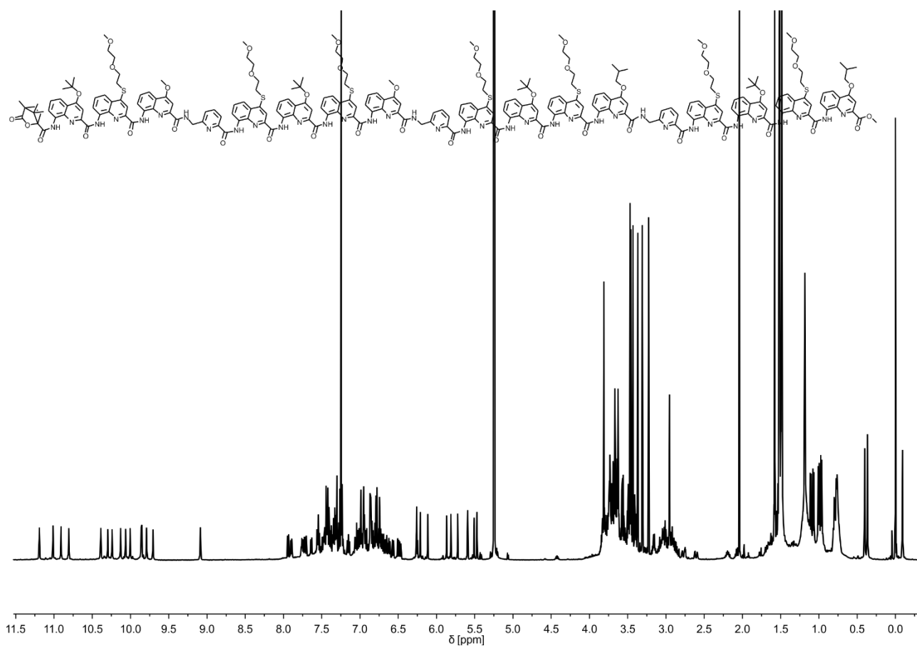
Figure S52. 1 H NMR spectrum (500 MHz, CD 2 Cl 2 ) of 15.
