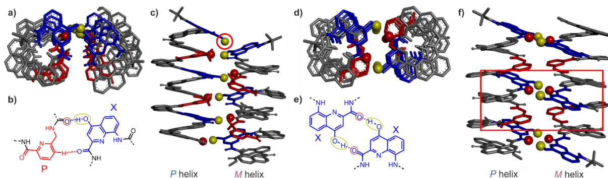
Figure S5. Energy minimized models of alternate, not experimentally observed hydrogen-bonded PM dimers. Top view (a) and side view (c) of an energy-minimized computational model [2] of 3 in a head-to-head PM shifted dimer arrangement (as opposed to the head-to-tail observed in the crystal). The prevalent hydrogen-bonding pattern is shown in (b). Here, one hydroxy group is not involved in hydrogen-bonding (encircled in red in c). Top view (d), side view (f) and hydrogen-bonding pattern (e) of an energy-minimized computational model [2] of a PM head-to-tail (not shifted) parallel arrangement of 3 as observed in a helix-turn-helix tertiary structure. [3] Here, two hydrogen bonds form every other helix turn, instead of one every helix turn in the shifted dimer. The hydrogen-bonding donors and acceptors are shown as yellow and red balls, respectively. The X units are shown in blue and the P Units in red tubes. Included solvent molecules, hydrogen atoms and side-chains are omitted for clarity.
