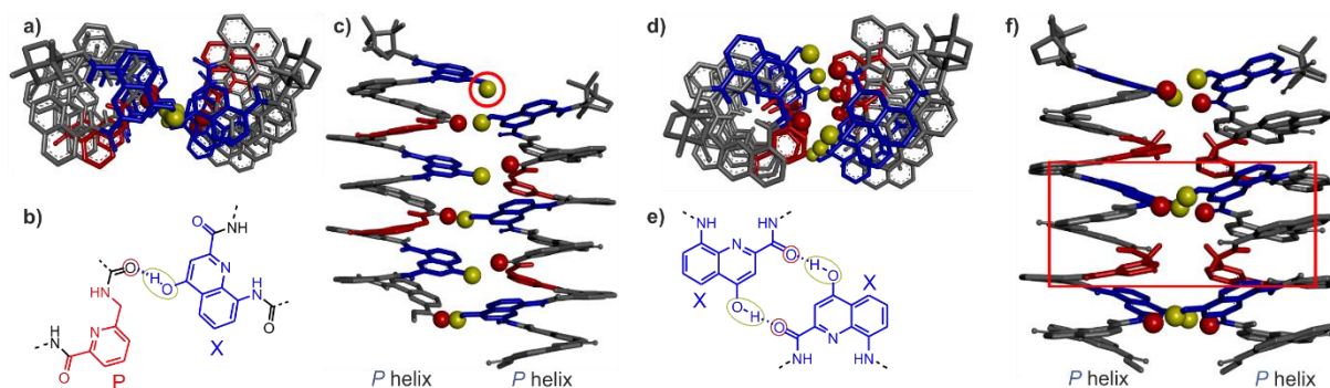
Figure S22. Energy minimized models of alternate, not experimentally observed hydrogen-bonded PP dimers. Top view (a) and side view (c) of an energy-minimized computational model [2] of 5 in a head-to-head PP shifted dimer arrangement (as opposed to the head-to-tail observed in the crystal). The prevalent hydrogen-bonding pattern is shown in (b). Here, one hydroxy group is not involved in hydrogen-bonding (encircled in red in c). Top view (d), side view (f) and hydrogen-bonding pattern (e) of an energy-minimized computational model [2] of a PP head-to-head (not shifted) parallel arrangement of 5 as observed in a helix-turn-helix tertiary structure. [1,3,4] Here, two hydrogen bonds form every other helix turn, instead of one every helix turn in the shifted dimer. The hydrogen-bonding donors and acceptors are shown as yellow and red balls, respectively. The X units are shown in blue and the P Units in red tubes. Included solvent molecules, hydrogen atoms and side-chains are omitted for clarity.
