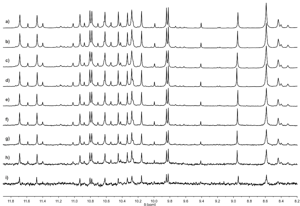
Figure S16. The proportions of the PM and PP/MM shifted dimers of 3 do not depend on concentration. Part of the 500 MHz ^1\text{H} NMR spectra of 3 ( \text{CD}_2\text{Cl}_2 , 25 °C) showing the amide and hydroxy proton resonances at 2.2 mM (a), 1.1 mM (b), 0.55 mM (c), 0.28 mM (d), 0.14 mM (e), 0.7 mM (f), 0.035 mM (g), 0.017 mM (h) and 0.009 mM (i). All spectra were measured after a two-week incubation time to reach equilibrium.
