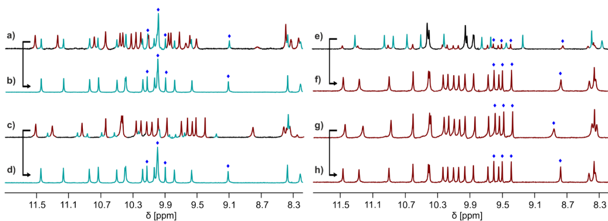
Figure S15. Control experiment to verify thermodynamic equilibrium is reached between the PM and PP/MM shifted dimers of 4 . Extracts of 500 MHz ^1\text{H} NMR-spectra of 4 (2.4 mM) at 25 °C in various solvents and after various equilibration times. a) Sample evaporated from an equilibrated \text{CD}_2\text{Cl}_2 solution, re-dissolved in \text{CDCl}_3 , and incubated for 2 days. b) Same sample after a three-week incubation. c) Sample evaporated from an equilibrated pyridine solution, re-dissolved in \text{CDCl}_3 , and incubated for 2 days. d) Same sample after a three-week incubation. e) Sample evaporated from an equilibrated \text{CDCl}_3 solution, re-dissolved in \text{CD}_2\text{Cl}_2 , and incubated for 1 day. f) same sample after a six-week incubation. g) sample evaporated from an equilibrated pyridine solution, re-dissolved in \text{CD}_2\text{Cl}_2 , and incubated for 2h. h) Same sample after a three-week incubation. The signals of two different species are marked with different colors.
