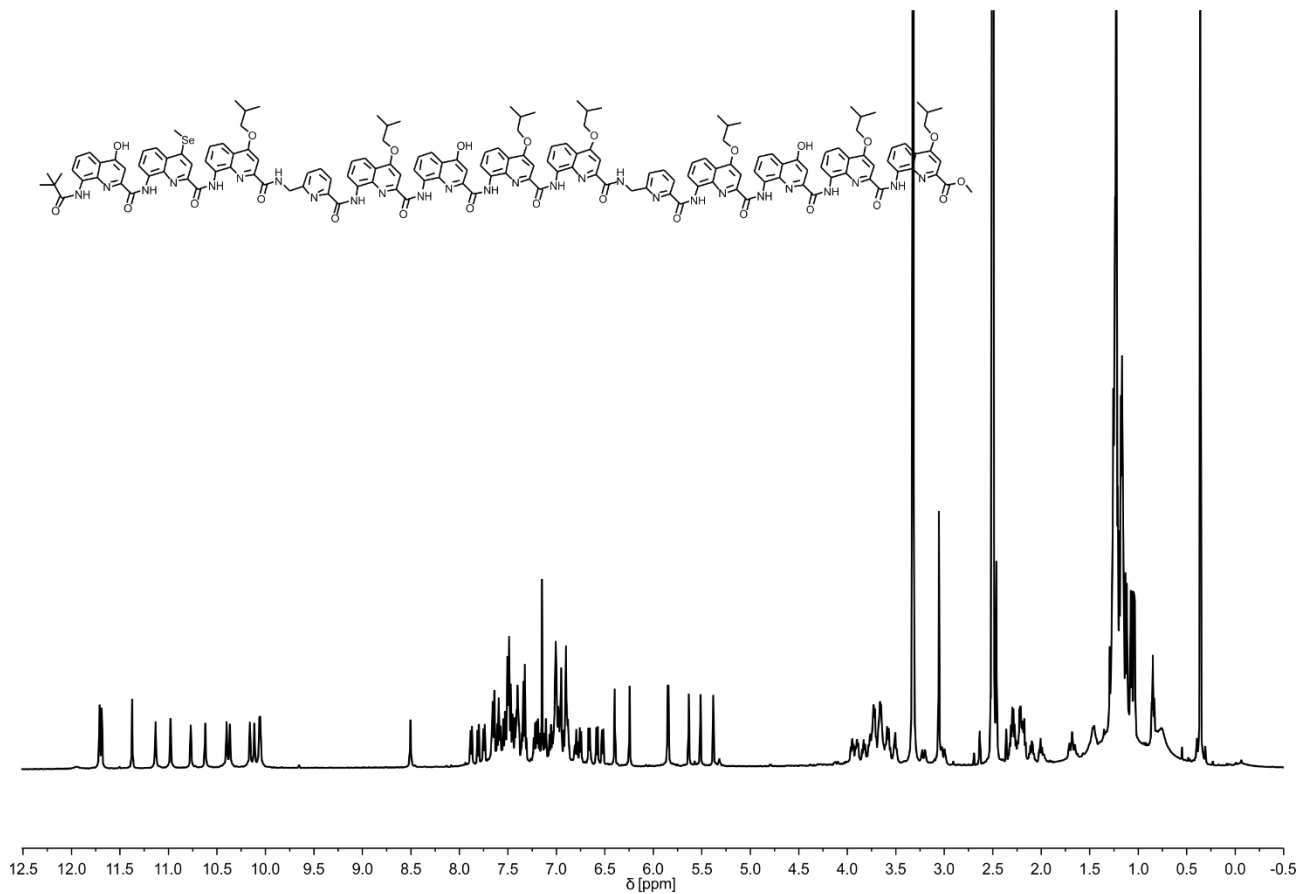
Figure S44. 1 H NMR spectrum (500 MHz, DMSO- d 6 ) of 3 .
