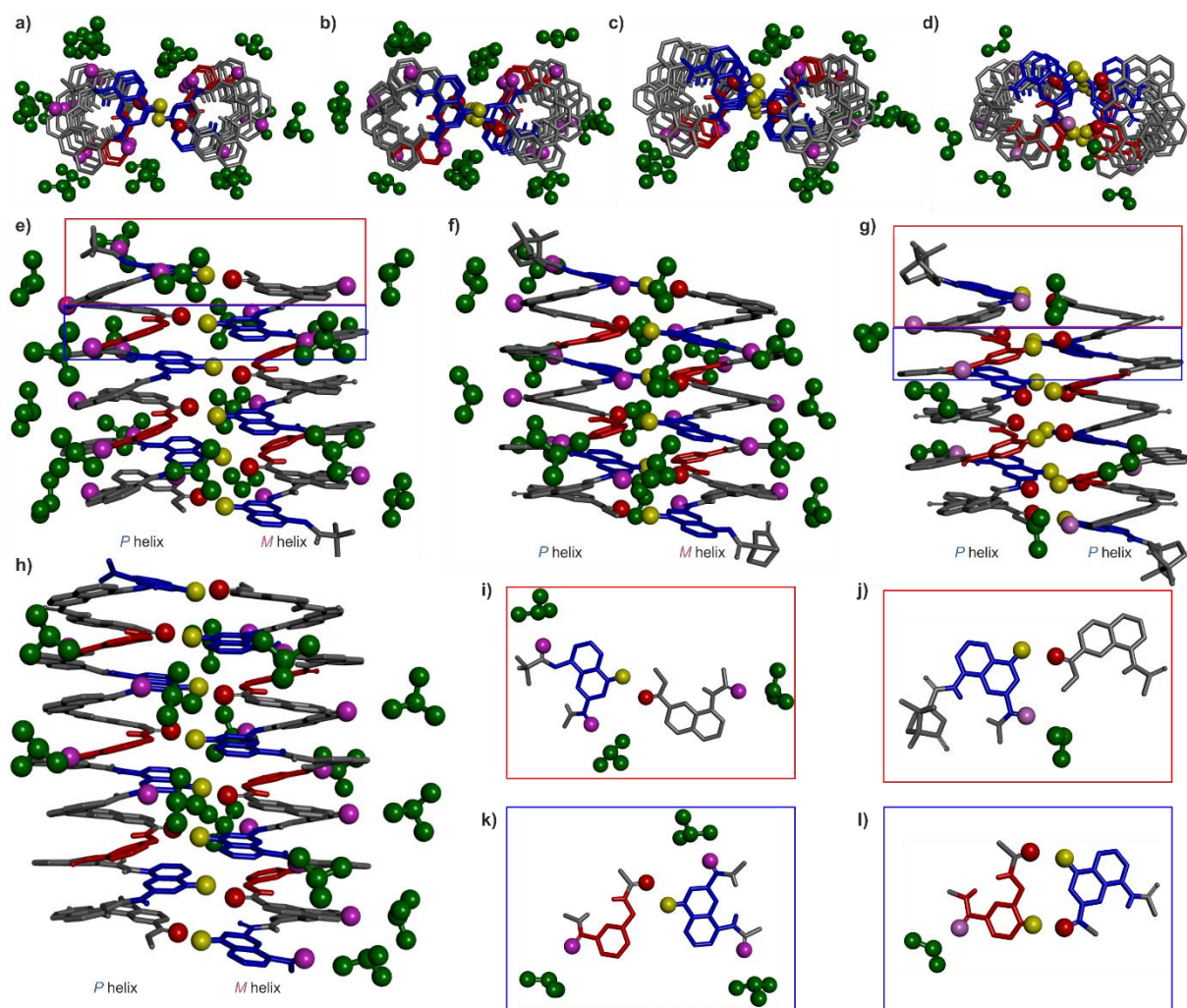
Figure S33. Almost all chloroform molecules hydrogen bond to amide carbonyl groups in solid state structures. Views of various solid state structures showing \text{CHCl}_3 or \text{CH}_2\text{Cl}_2 solvent molecules in the crystal lattice. Top views of the PM shifted dimers of 3 (a), 5 (b) and 7 (c) with \text{CHCl}_3 molecules, and top view of the chiral shifted dimer of 5 (d) with \text{CH}_2\text{Cl}_2 molecules. Side views of the PM shifted dimers of 3 (e), 5 (f) and 7 (h) with \text{CHCl}_3 molecules, and side view of the chiral shifted dimer of 5 (g) with \text{CH}_2\text{Cl}_2 molecules. Slices of the dimers showing the solvent molecules surrounding the X, P or Q units are shown in i)-k). i) and k) are from the structure of 3 with \text{CHCl}_3 molecules (red and blue boxes in e). j) and l) are from the structure of 5 with \text{CH}_2\text{Cl}_2 molecules (red and blue boxes in g). The hydrogen-bonding donor and acceptor sites are shown as yellow and red balls, respectively. Carbonyl groups binding to \text{CHCl}_3 or \text{CH}_2\text{Cl}_2 molecules are shown as pink balls. \text{CHCl}_3 and \text{CH}_2\text{Cl}_2 molecules are shown as green balls. The X units are shown in blue and the P Units in red tubes. Hydrogen atoms and side-chains are omitted for clarity.
