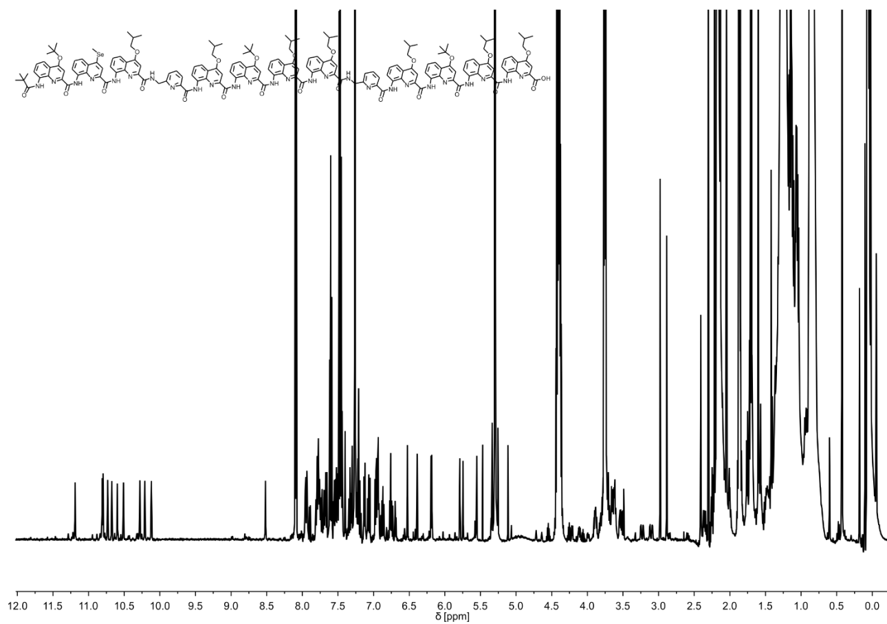
Figure S42. 1 H NMR spectrum (500 MHz, CDCl 3 ) of 8 .
