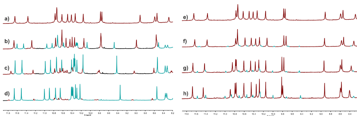
Figure S10. Interconversion of the PM and PP/MM shifted dimers of 3 upon changing \text{CDCl}_3/(\text{CD}_2\text{Cl})_2/\text{CD}_2\text{Cl}_2 solvent mixtures. a)-d) Part of the 500 MHz ^1\text{H} NMR spectra of 3 (2.4 mM in \text{CDCl}_3/(\text{CD}_2\text{Cl})_2 mixtures) at 25 °C showing the amide and hydroxy proton resonances. The volume percentages of (\text{CD}_2\text{Cl})_2 are 100 (a), 75 (b), 50 (c), 25 (d). e)-f) Part of the ^1\text{H} NMR spectra (500 MHz, 25 °C) showing the amide and hydroxy proton resonances of 3 , 2.4 mM in \text{CD}_2\text{Cl}_2/(\text{CD}_2\text{Cl})_2 . The volume percentages of (\text{CD}_2\text{Cl})_2 are 100 (e), 75 (f), 50 (g), and 25 (h). The signals of two different species are marked with different colors. Signals of the species dominant in \text{CHCl}_3 ( PM shifted dimer) are marked in turquoise, those of the species dominant in \text{CH}_2\text{Cl}_2 ( PP/MM shifted dimer) are marked in brown. All spectra were measured after a 2h incubation time to reach equilibrium.
